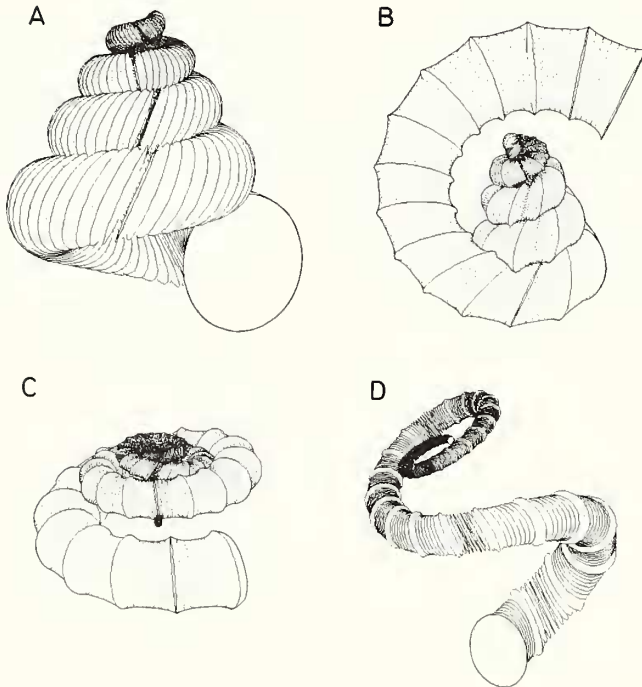
TEXT-FIG. 10. Computer-graphics showing the theoretical rib obliquity with constant aperture angle. A, Eubostrychoceras muramotoi Matsumoto. B, Ainoceras kamuy Matsumoto and Kanie. C, Muramotoceras yezoense Matsumoto. D, E. japonicum (Yabe). The aperture angles of these species are set at 40°, 60°, 40°, and 40° respectively.
